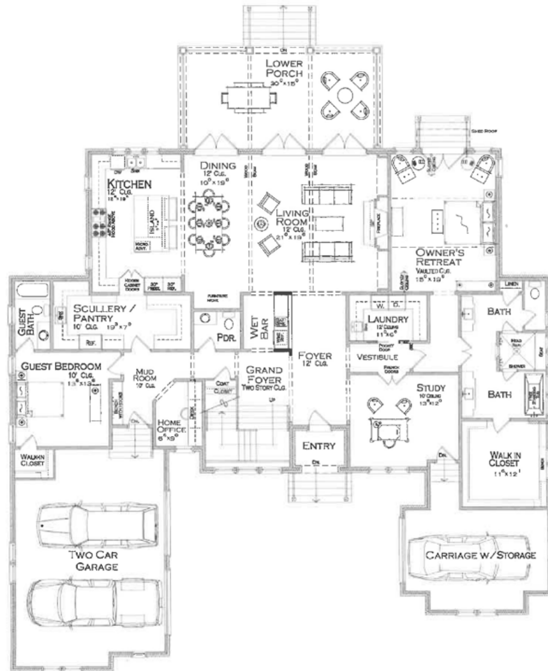
Main Level
